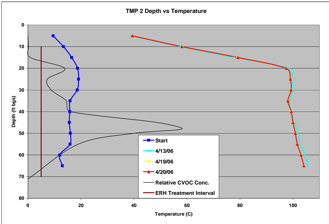
Figure 5. Subsurface Temperature at Depth vs Relative CVOC Concentration at TMAP 2
