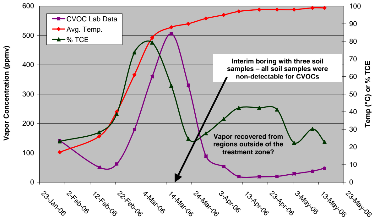
Figure 10. Recovery of Total CVOC (purple line) vs TCE (green line) with Temperature over Time
