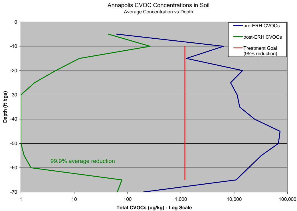
Figure 11. Average Concentrations of Total CVOCs at Depth Pre and Post ERH
