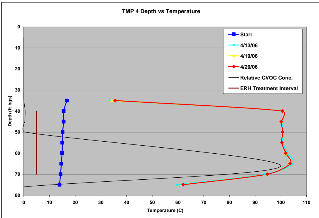
Figure 6. Subsurface Temperature at Depth vs Relative CVOC Concentration at TMAP 4
