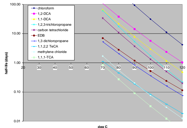
Figure 1. Hydrolysis of Halogenated Alkanes at Elevated Temperatures
