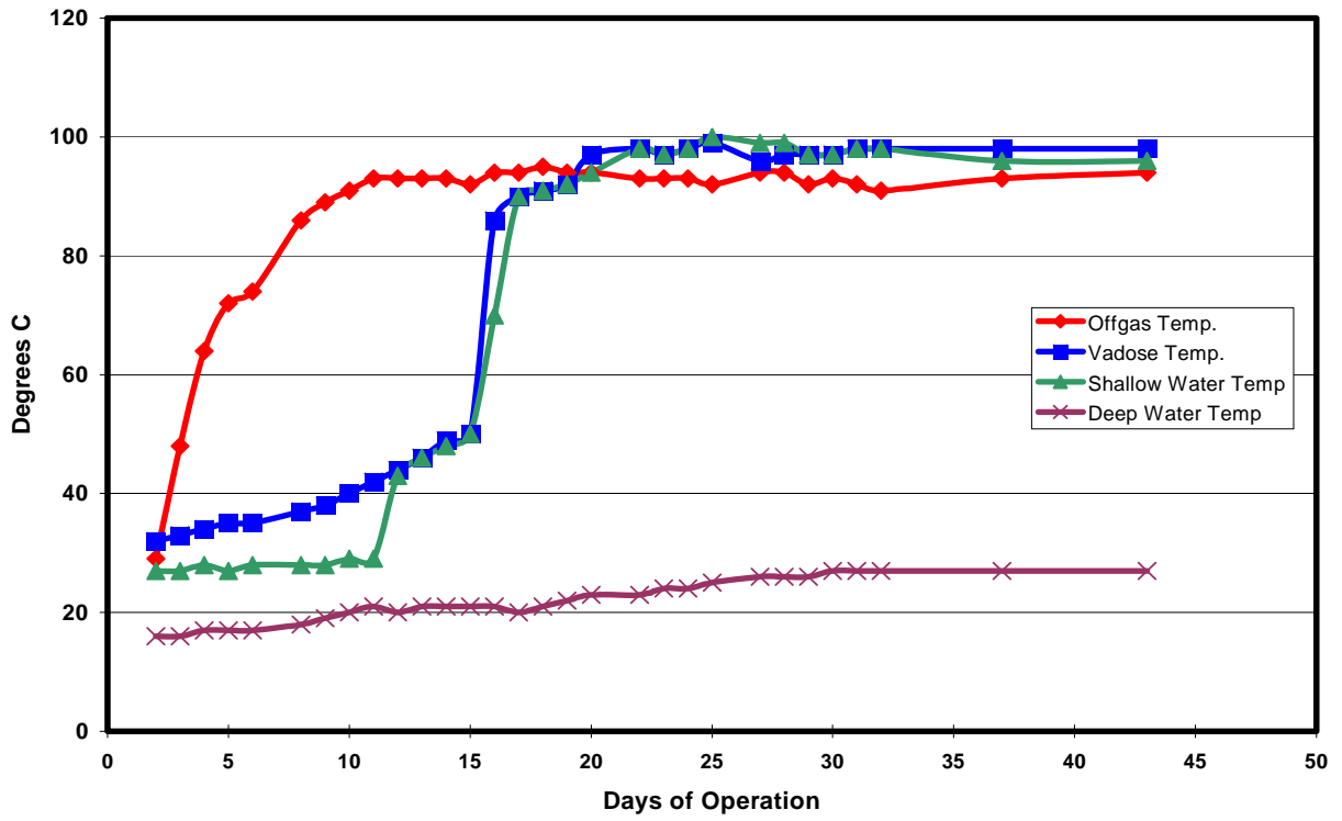
Figure 1. Temperature Vs Days of Operation
