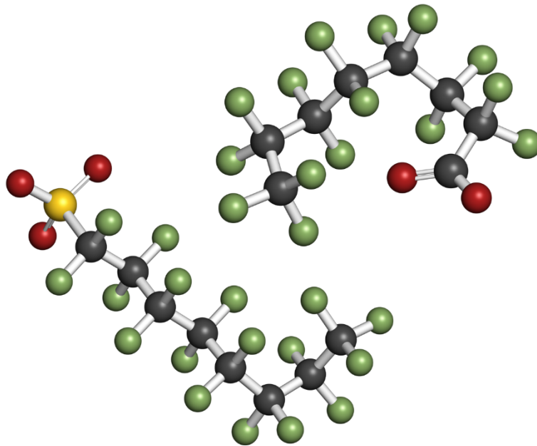
Figure 1: PFOA and PFOS Molecules
