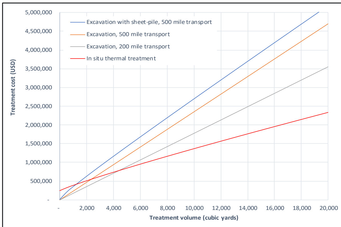
Figure 1: Estimated treatment costs as a function of final volume for a typical TCE site with treatment to 40 ft bgs. Assumed disposal and excavation costs are $100/cy and $15/cy, respectively.
